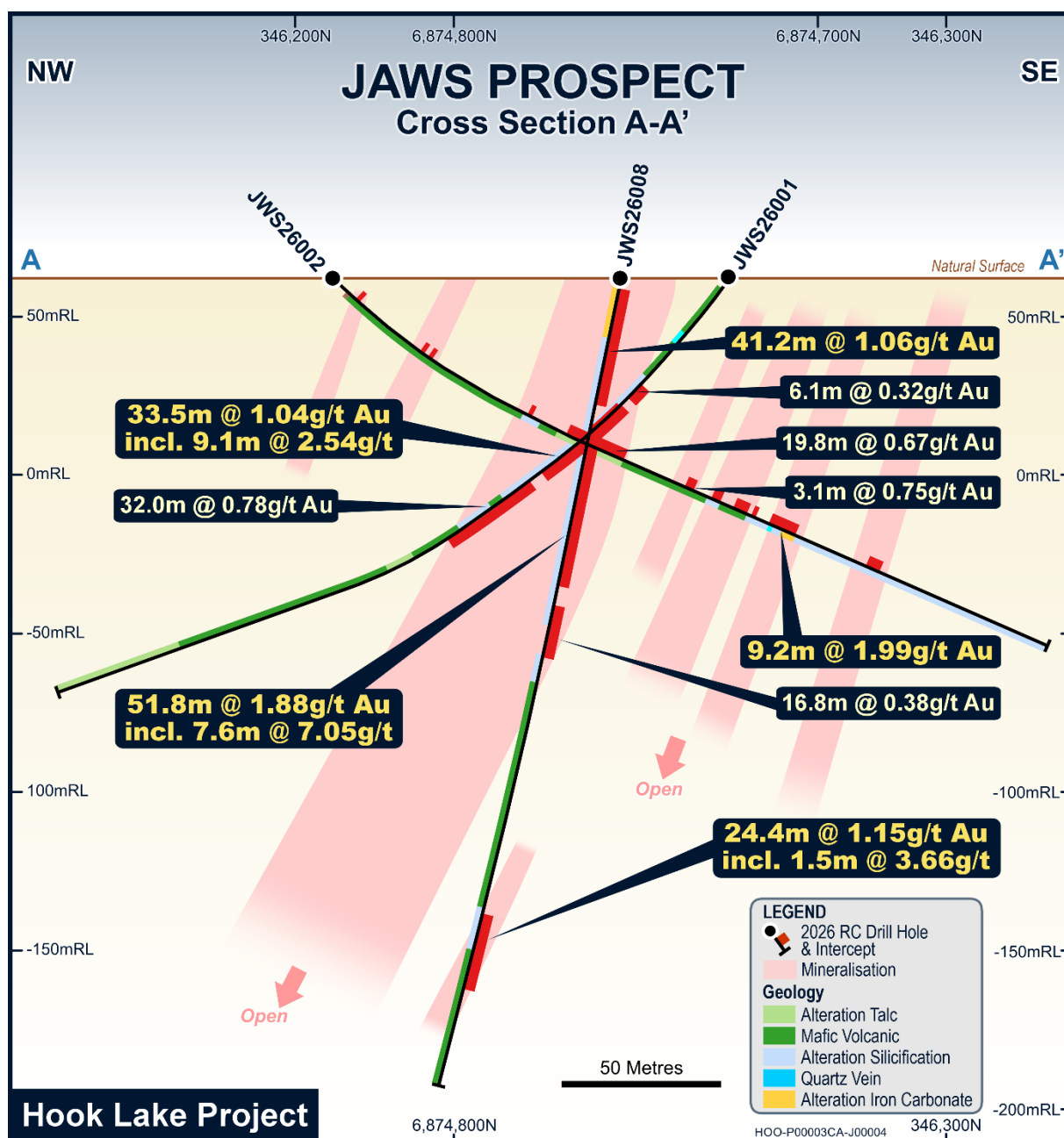
Figure 4: Drillhole cross section showing the mineralisation encountered downhole in JWS26008.
